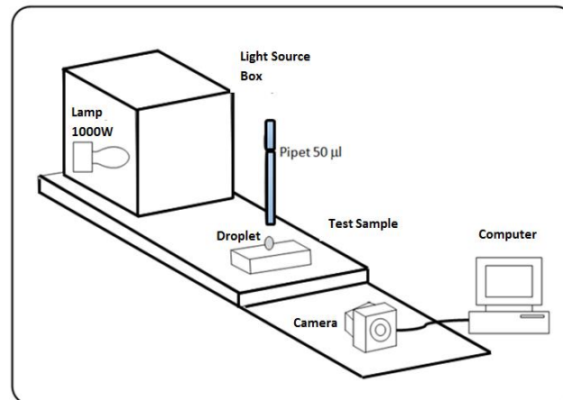
Figure 1 Equipment for surface contact angle measurements
